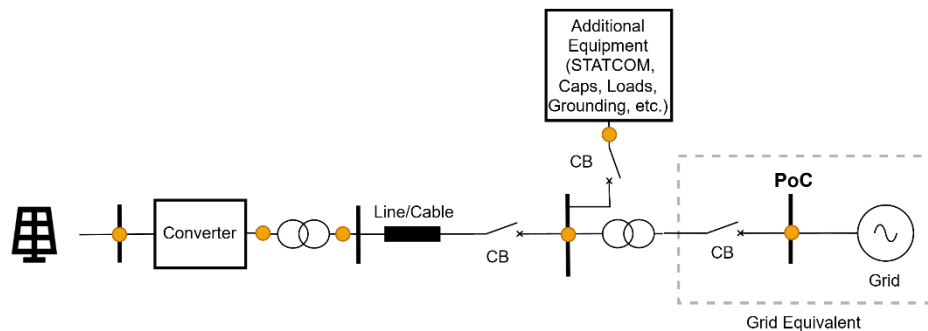
Figure 5: Measurement nodes in the EMT model
