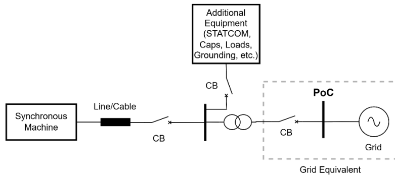
Figure 2: Layer 2 of the EMT model structure
