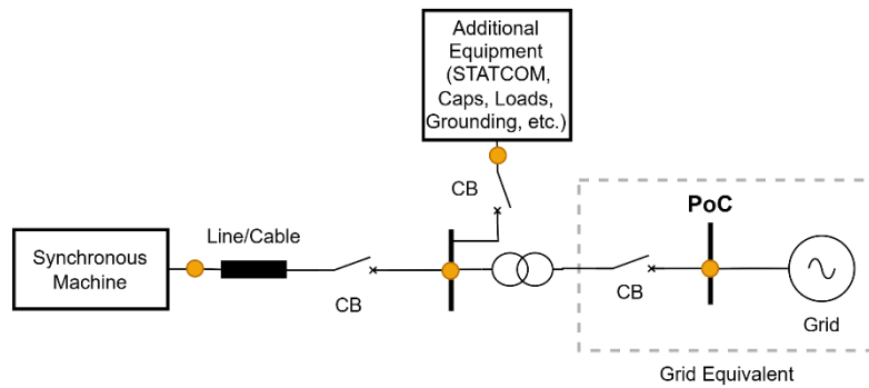
Figure 3: Measurement nodes in the EMT model
