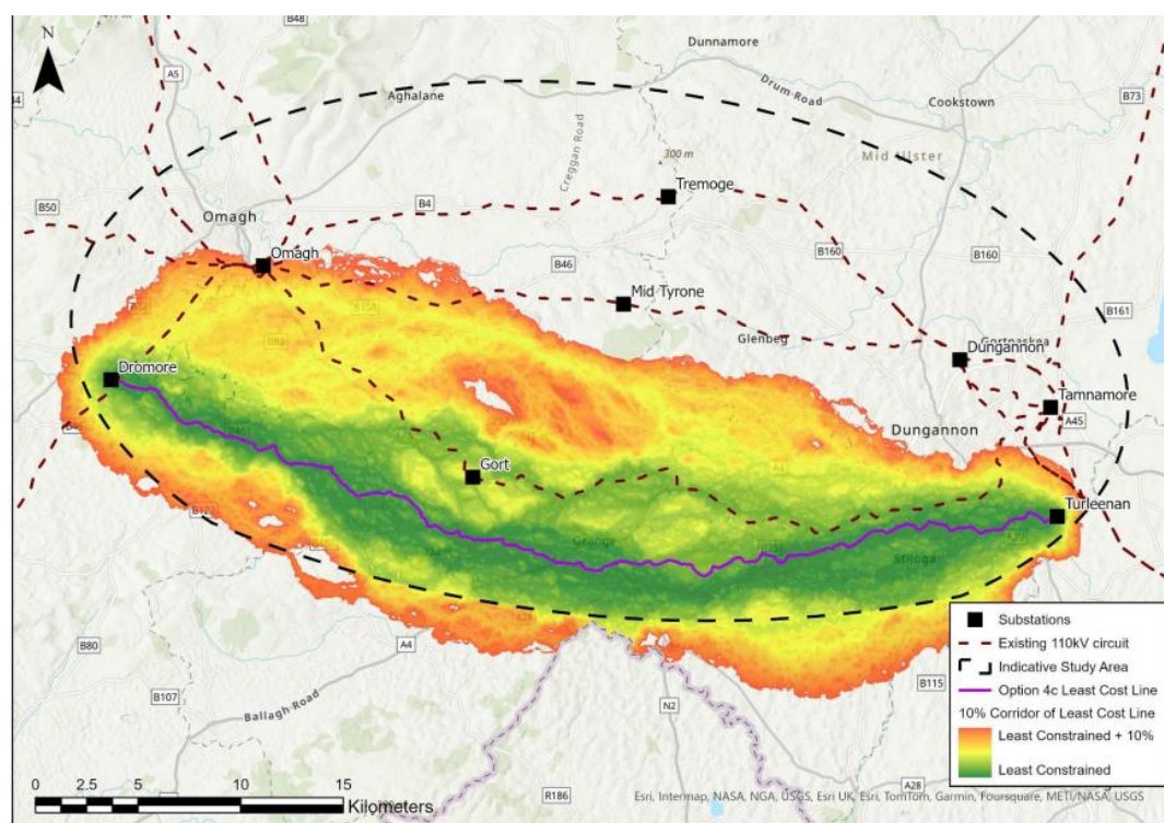
Figure 6.6: Indicative environmental constraints for Option 3C
