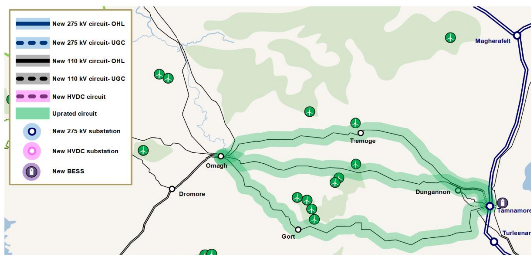
Figure 3.6: Illustrative configuration of Option 2C
