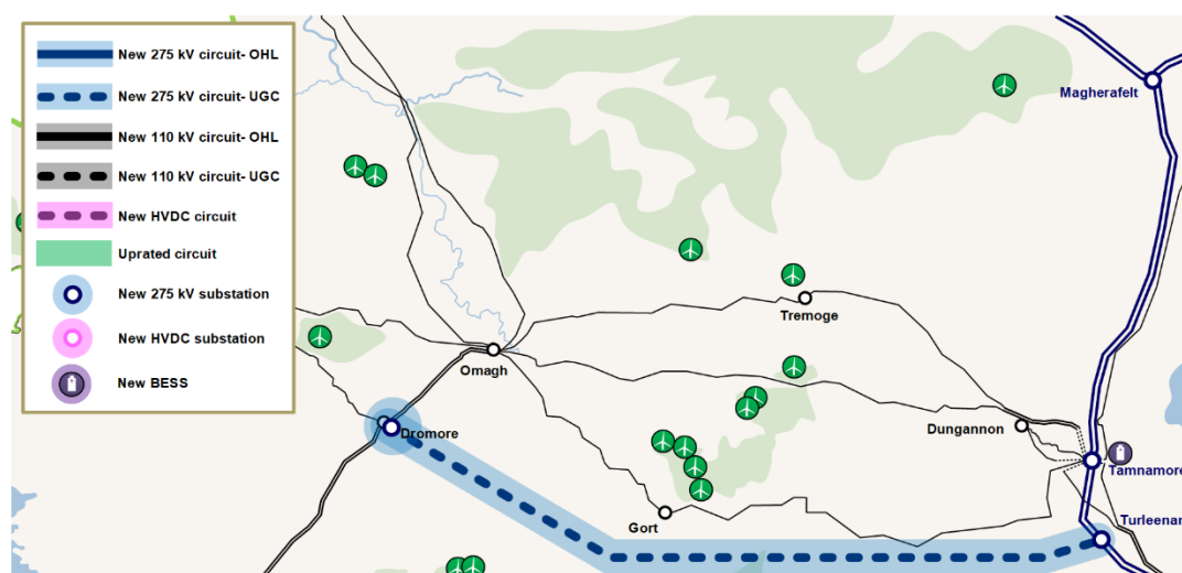
Figure 3.9: Illustrative configuration of Option 3C
