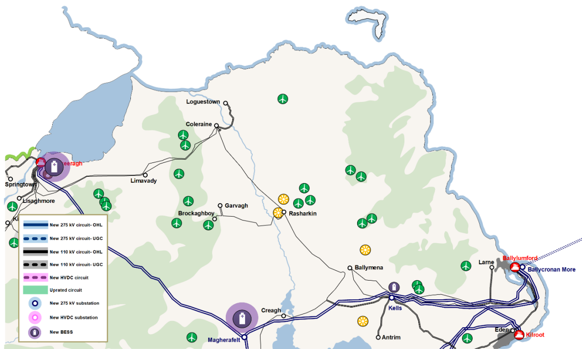
Figure 3.10: Illustrative configuration of Option 4
