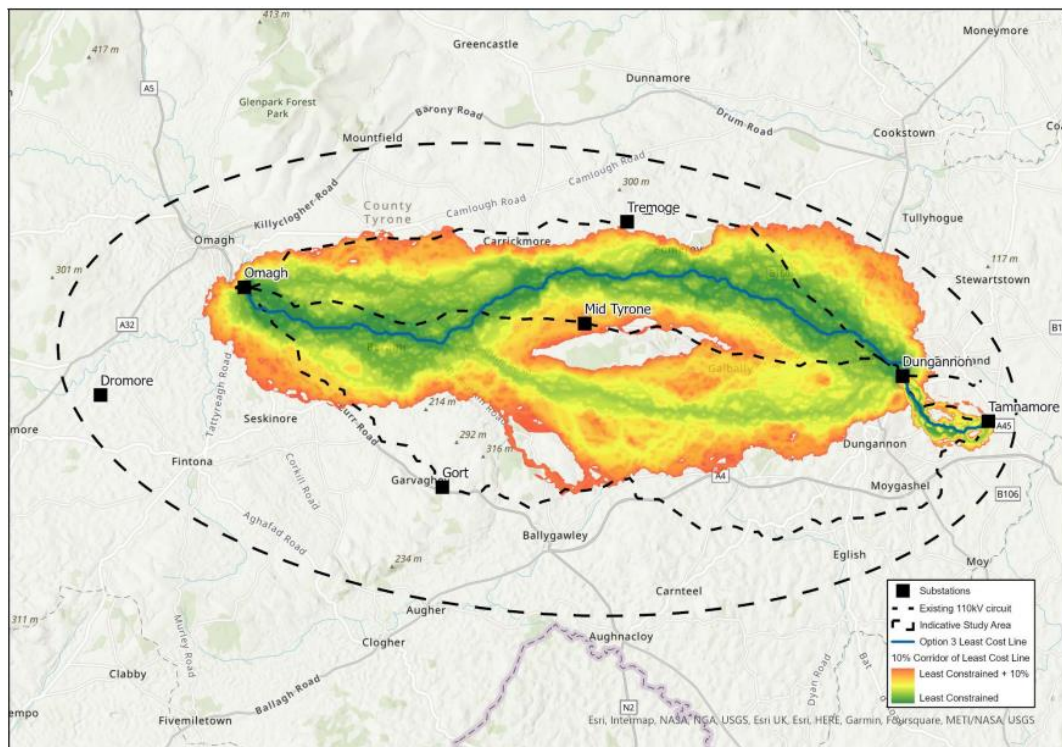
Figure 6.3: Indicative least constrained environmental line for Option 2B
