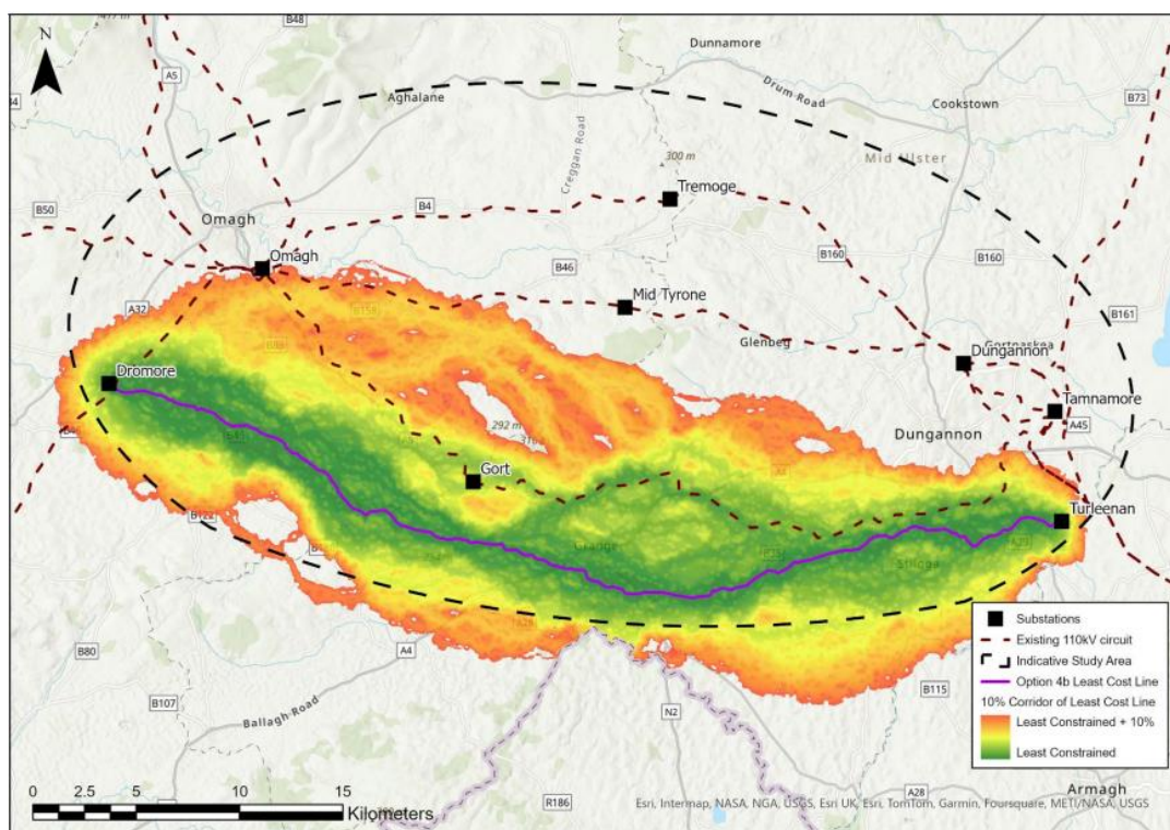
Figure 6.5: Indicative environmental constraints for Option 3B
