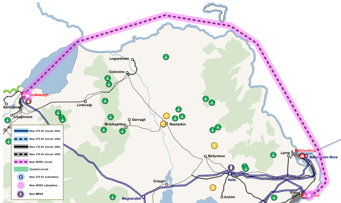
Figure 3.1: Illustrative configuration of Option 1A
