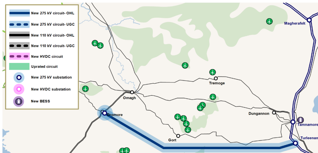
Figure 3.8: Illustrative configuration of Option 3B
