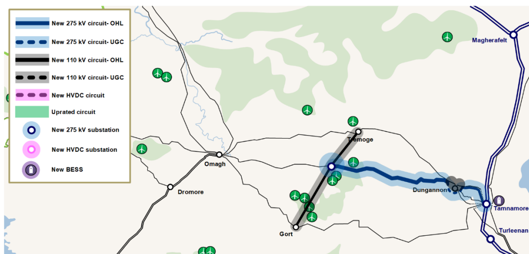
Figure 3.4: Illustrative configuration of Option 2A
