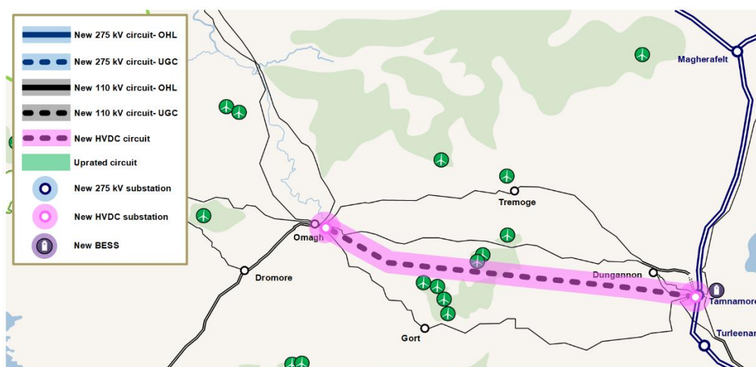
Figure 3.3: Illustrative configuration of Option 1C
