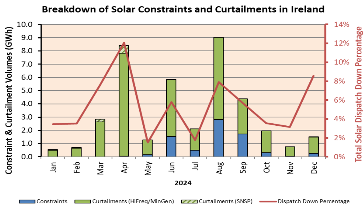
Figure 15: Monthly breakdown of the main solar dispatch-down categories in Ireland in 2024
