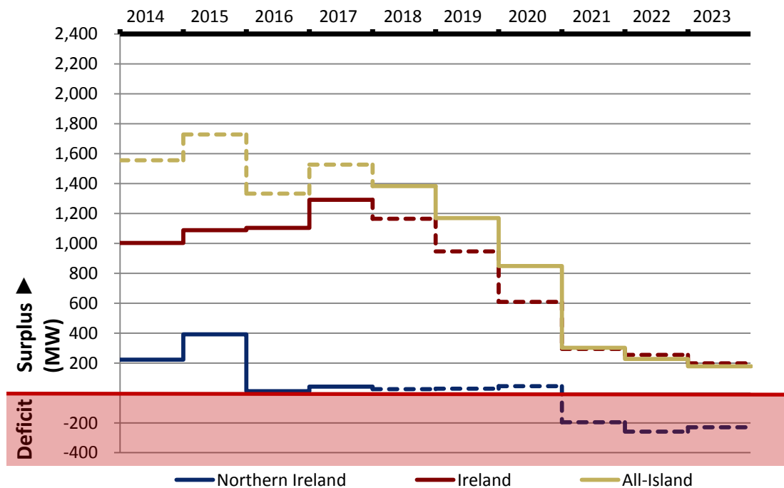
Figure 4-2 The adequacy situation without the interconnectors to Great Britain
