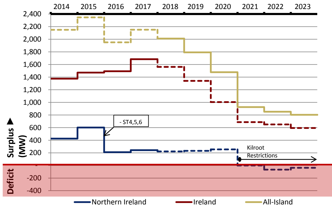
Figure 4-1 Adequacy results for the Base Case scenario, shown for Ireland, Northern Ireland and on an all-island basis.
