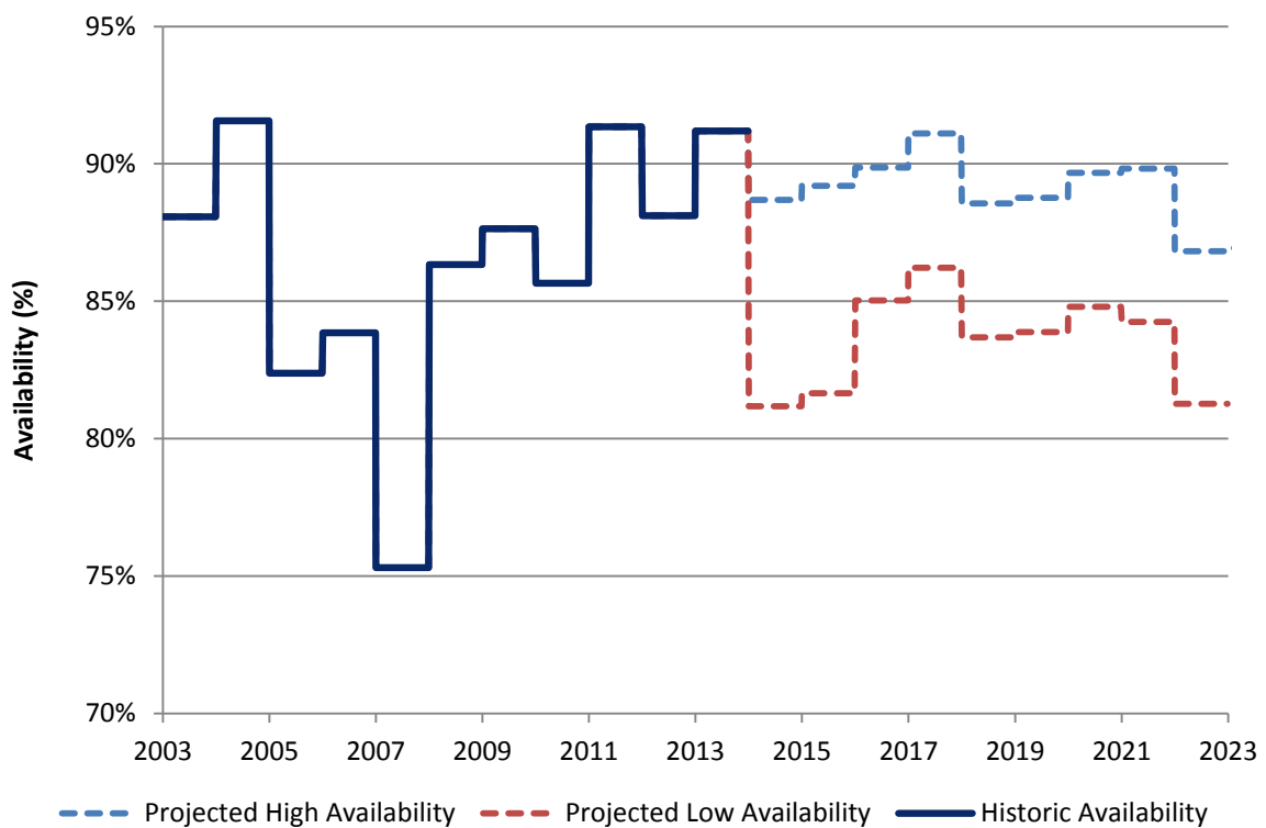
Figure 3-11 Historical and predicted Plant Availabilities in Northern Ireland (without Moyle)
