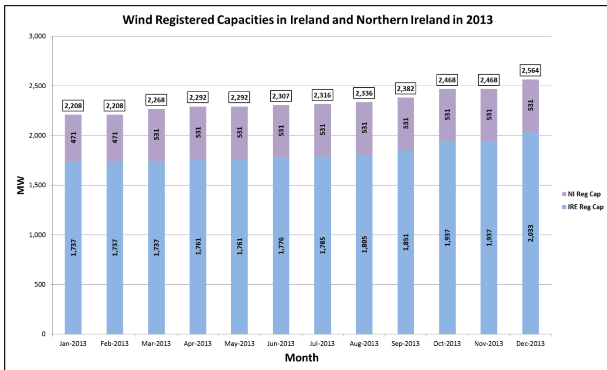
Figure 2: All-Island Monthly Wind Registered Capacities in 2013
