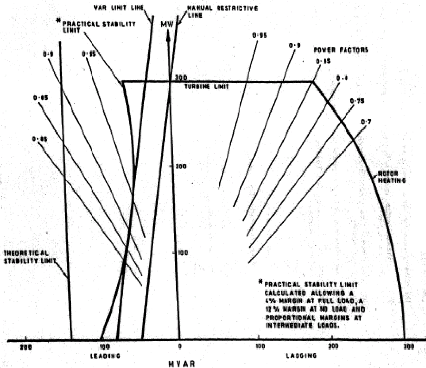
CAPABILITY CHART KOA 1.2 (KCA 1.2)
