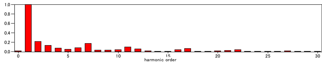
Fig. A1-38 Frequency component spectrum of the switching waveform at Woodland 220 kV bus (phase to earth).
