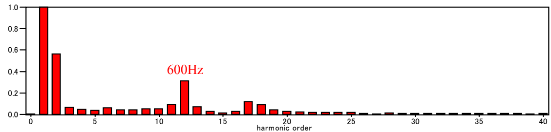
Fig. A1-14 Frequency component spectrum of the switching waveform at the 220 kV cable open end (phase to earth).
