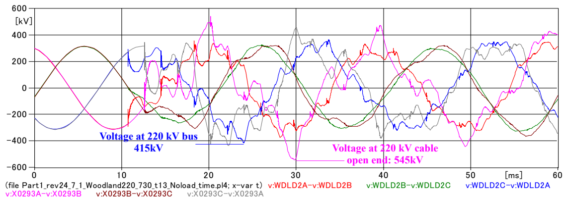
Fig. A1-37 Switching waveforms at the Woodland 220 kV bus and 220 kV cable open end (phase to phase).
