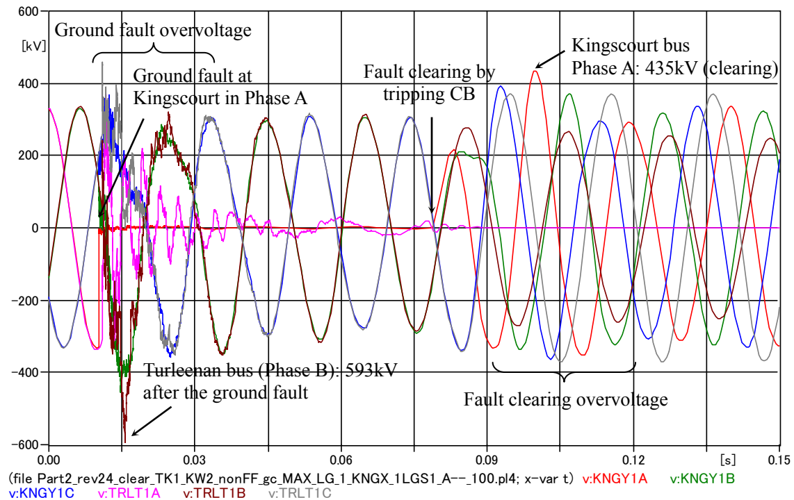
Fig. 5.10 Waveform of the maximum overvoltage.
