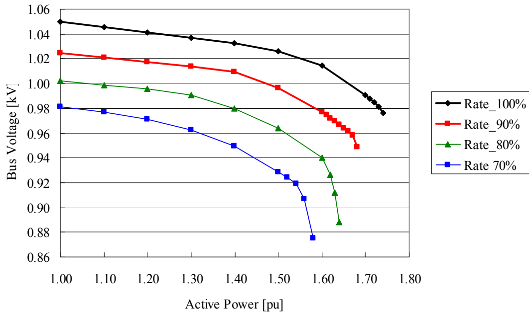
Fig. 6-9 PV-curves at the Cahir 400 kV bus with the loss of the 400 kV Cahir - Aghada line.
