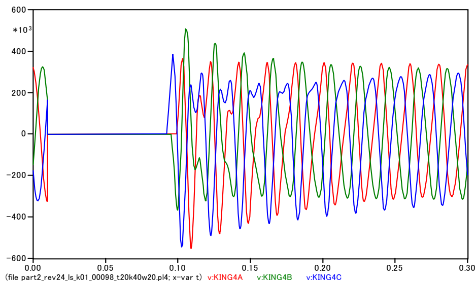
Fig. 4.33 Overvoltage caused by islanding under the smallest impedance value of Turleenan. (dummy source impedance at Turleenan 275 kV: 20 mH)
