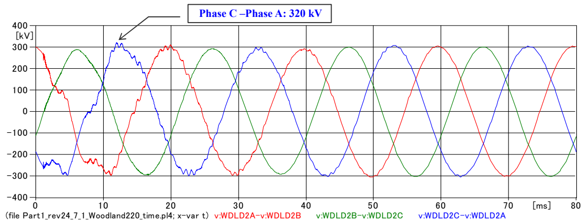
Fig. 4-8 Waveforms of the switching overvoltage at the Woodland 220 kV bus (phase to phase).
