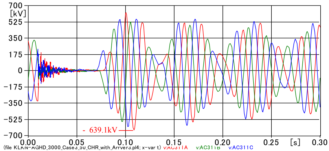
Fig. 4-92 Waveform of the highest overvoltage with arresters at Aghada S/S in Case B2 (approx. 100% compensation).
