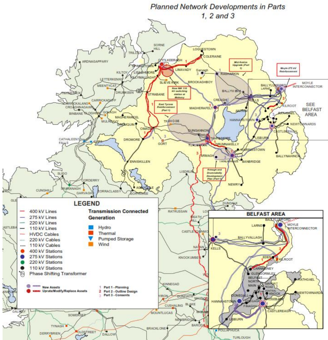
Figure 6-1 Planned Network Developments in Parts 1, 2 and 3 (not including NW of NI Reinforcement)
